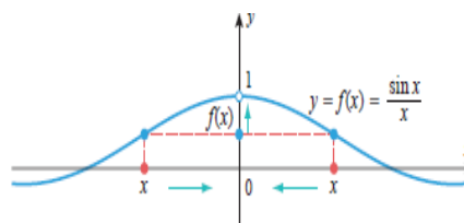
Figure 3.5: Limit x \rightarrow 0 when f(x) is not defined at x = 0
