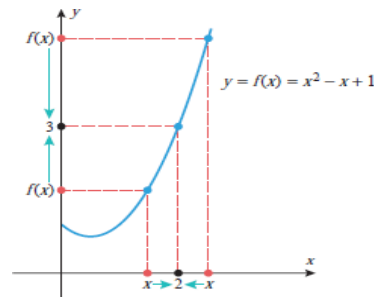
Figure 3.3: Limit x \rightarrow 2
