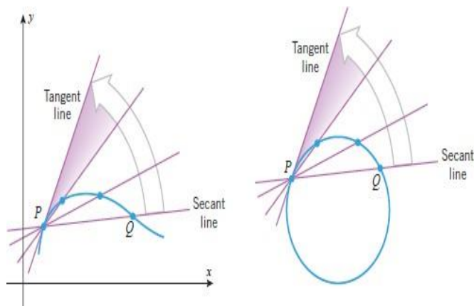
Figure 3.1: Tangent line as a limit of secant line
