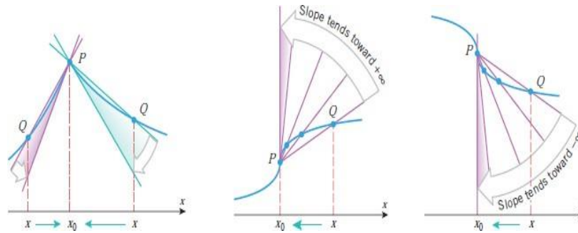
Figure 4.1: The tangent lines
