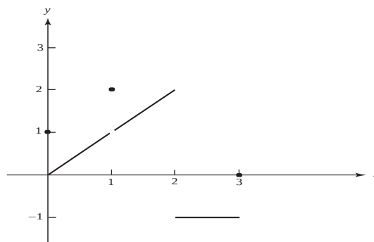
Figure 3.8: Graph of the function
