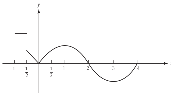
Figure 4.2: Extreme values of a function
