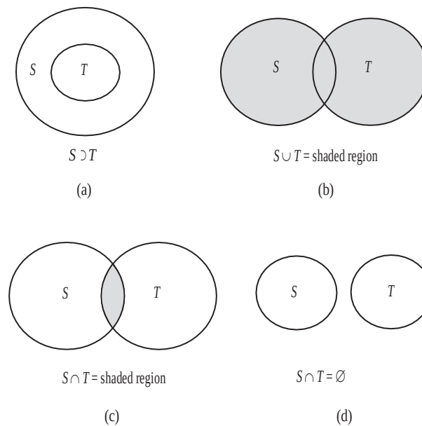
Figure 1.1: (a) Subset (b) Union of two sets (c) Intersection of two sets, (d) Disjoint sets
