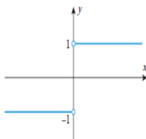
Figure 3.6: Limit x \rightarrow 0
