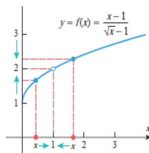
Figure 3.4: Limit x \rightarrow 1 when f(x) is not defined at x = 1
