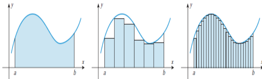
Figure 5.1: Area under the curve
