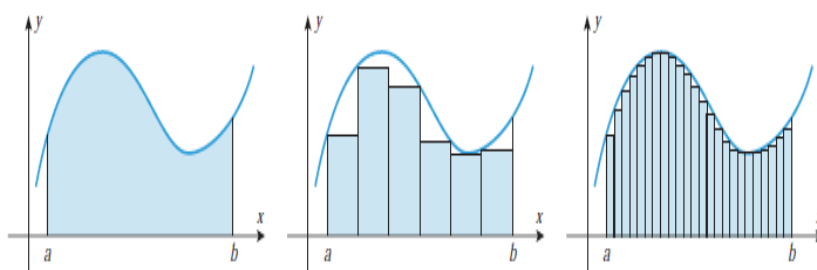
Figure 3.2: Area under the curve as limit
