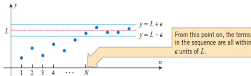
Figure 2.1: Convergence of the sequence
