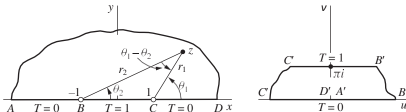
FIGURE 140 w = \log \frac{z-1}{z+1} \mu , \frac{r_1}{r_2} > 0 , -\frac{\pi}{2} < \vartheta_1 - \vartheta_2 < \frac{3\pi}{2} .
