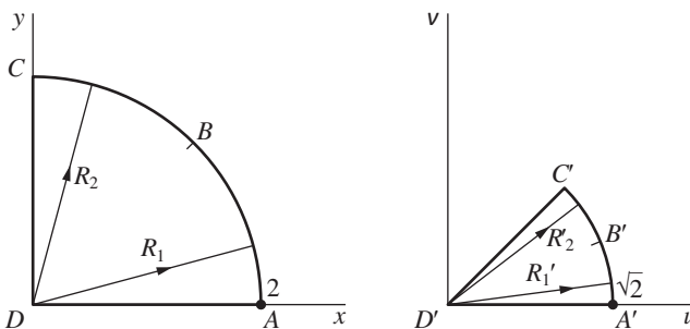
FIGURE 123 w = F_0(z) .
