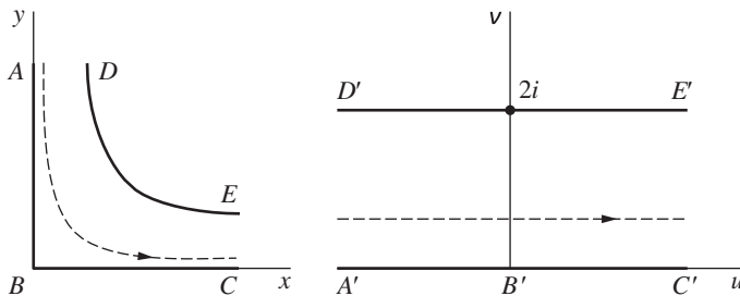
FIGURE 18 w = z^2 .
