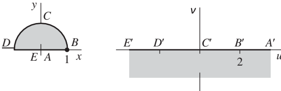
FIGURE 16 w = z + \frac{1}{z}.
