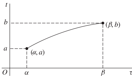
FIGURE 37 t = \varphi(\tau)
