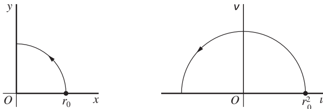
FIGURE 19 w = z^2
