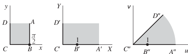
FIGURE 124 w = F_0(\sin z) .
