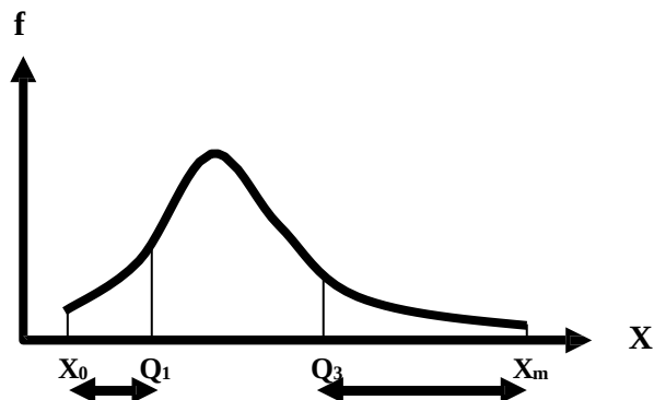
THE POSITIVELY SKEWED CURVE
