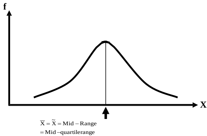
THE SYMMETRIC CURVE
