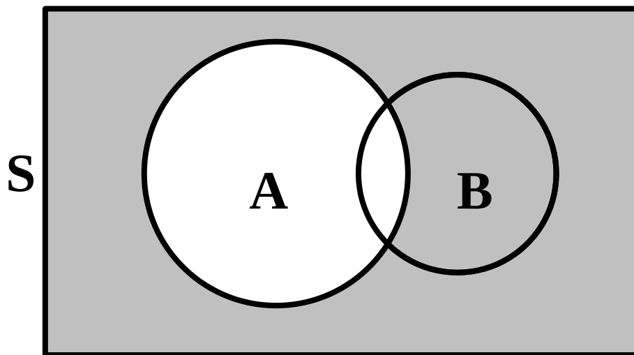
\bar{A} is shaded
