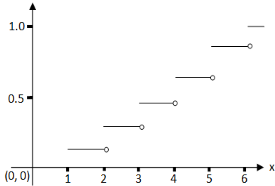
Figure 1: Distribution Function
