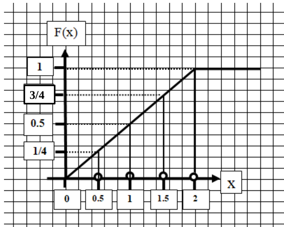
Figure 2: Distribution Function
