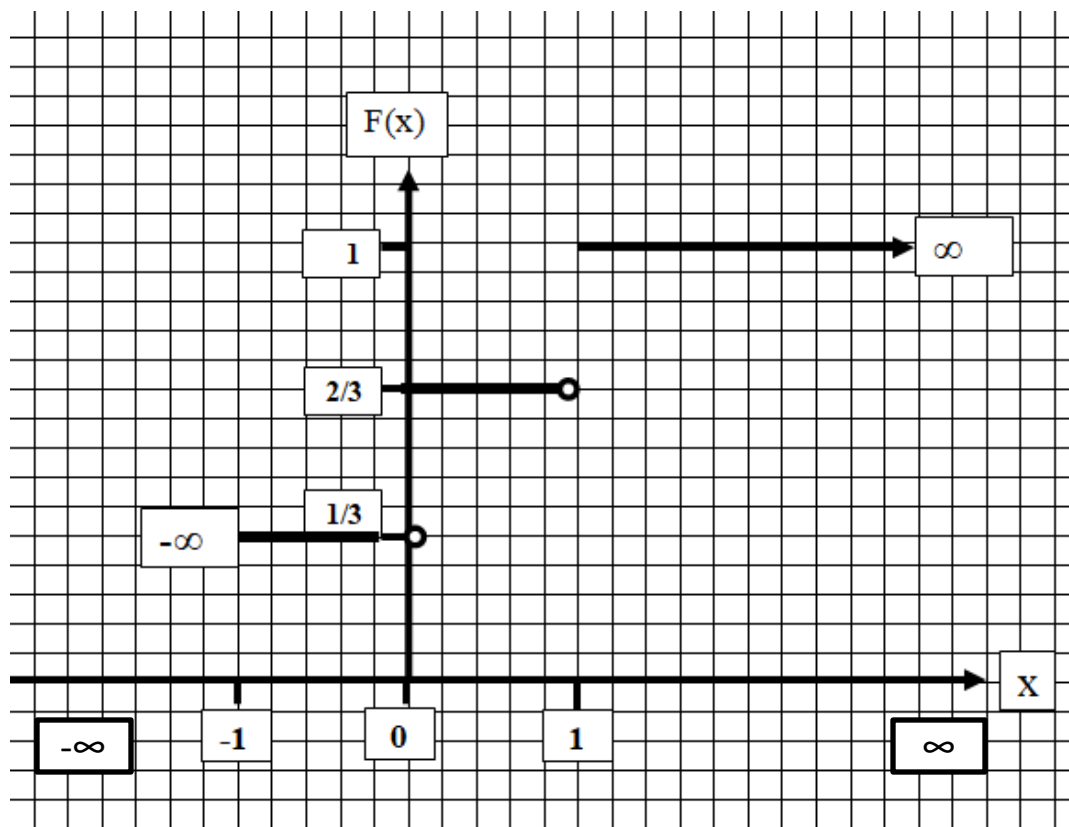
Figure 1: Distribution Function
