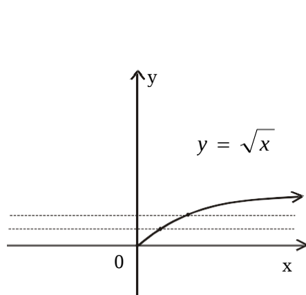
ONE-TO-ONE FUNCTION from \mathbb{R}^+ to \mathbb{R}
