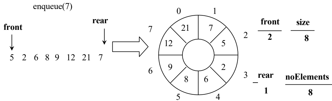
Fig 14. Another element added in circular array
