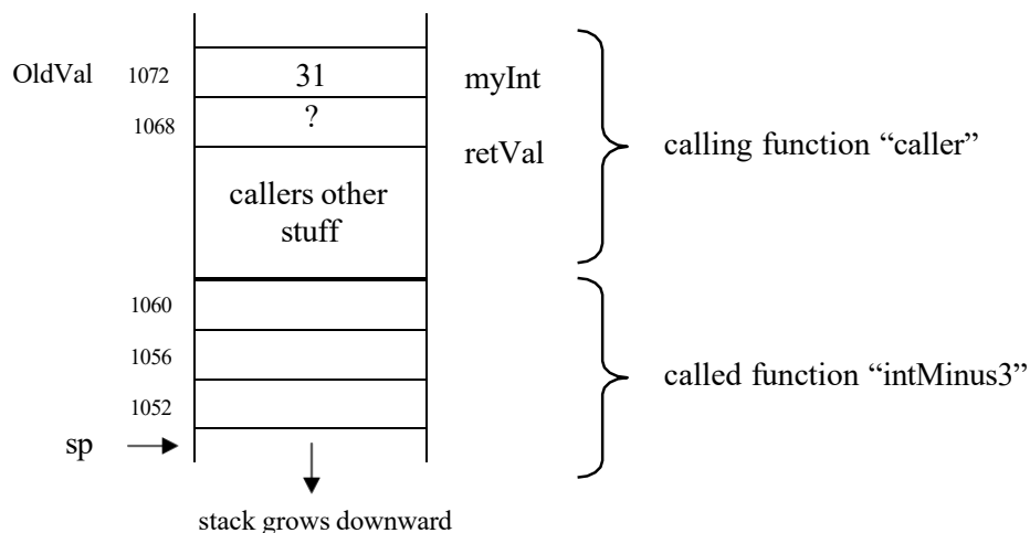
Fig 17.10: call stack when intMinus3 is called
