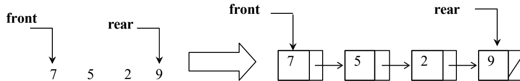
Fig 5. Insertion of one element using enqueue(9)
