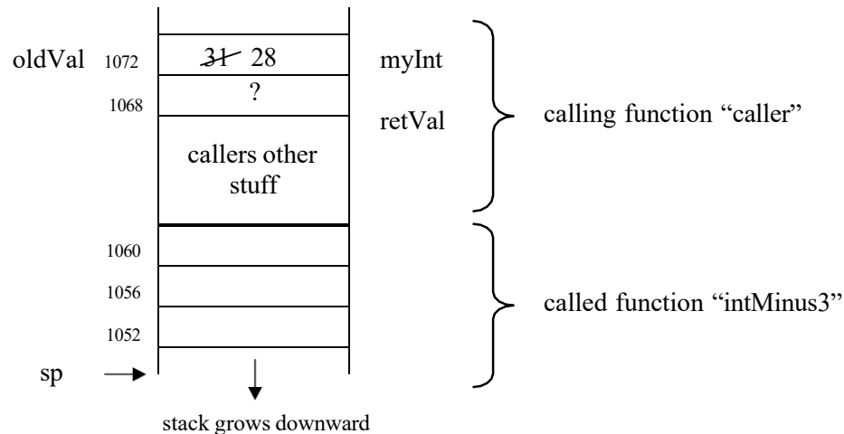
Fig 17.11: call stack layout after oldVal = oldVal - 3 ;
