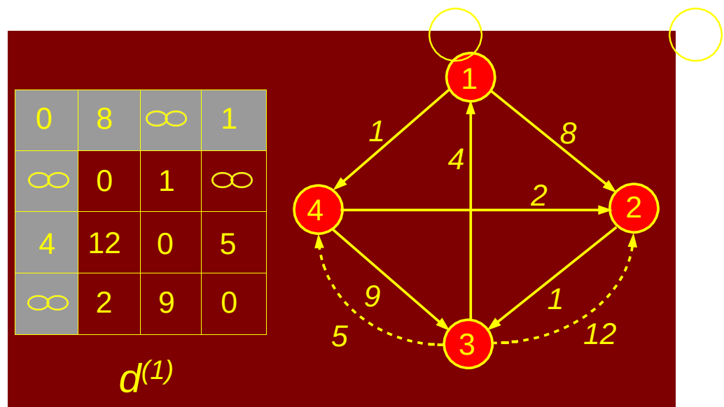
Figure 8.78: Floyd-Warshall Algorithm example: d^{(1)}
