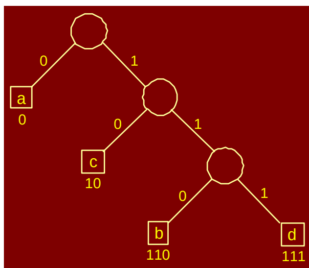
Figure 7.1: Huffman binary tree for the string “abacdaaac”
