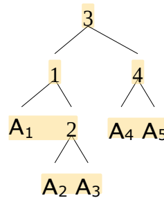
Figure 6.2: Optimum matrix multiplication order for the five matrices example
