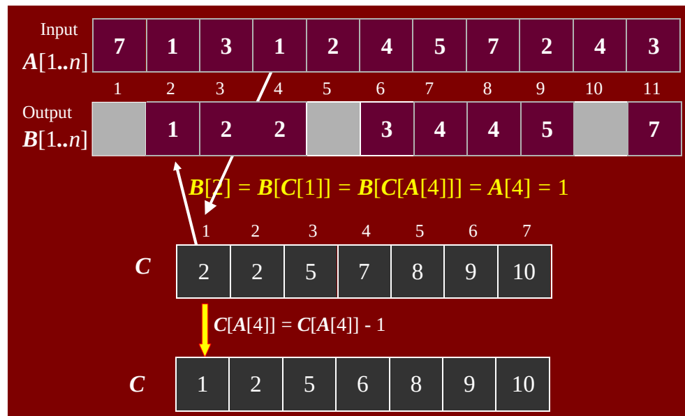
Figure 5.16: A[4] placed in output array B
