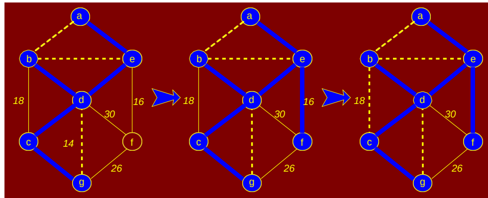
Figure 8.54: Kruskal algorithm: (e, f) added
