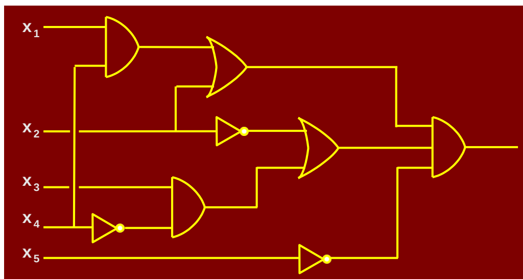
Figure 9.9: Logical circuit for a boolean formula
