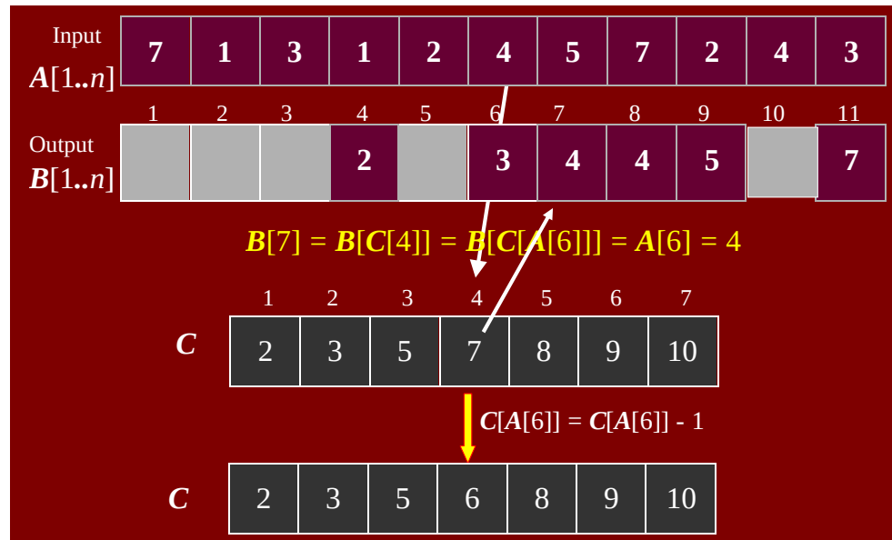
Figure 5.14: A[6] placed in output array B
