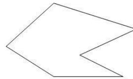
Simple Polygon
