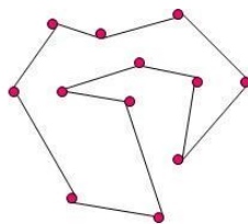
Simple Polygon
