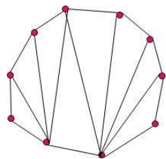
Triangulation
