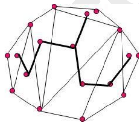
Dual Graph
