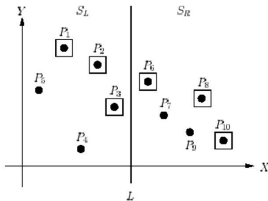
The maximal points of S_L and S_R
