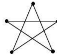
hamiltonian
