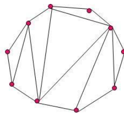
Triangulation
