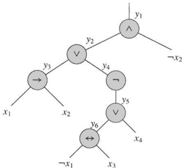
Figure 34.11 The tree corresponding to the formula \phi = ((x_1 \rightarrow x_2) \vee \neg((\neg x_1 \leftrightarrow x_3) \vee x_4)) \wedge \neg x_2 .
