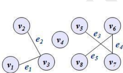
The Graph, G
