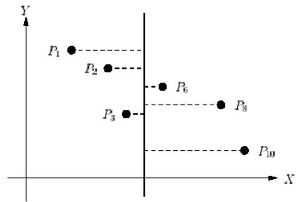
P_3 is not maximal point of S_L
