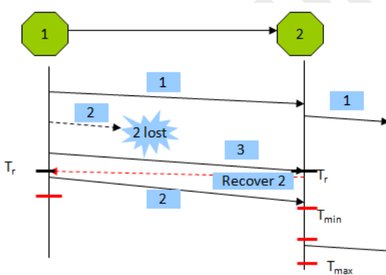
PSFQ Fetch Operation.
