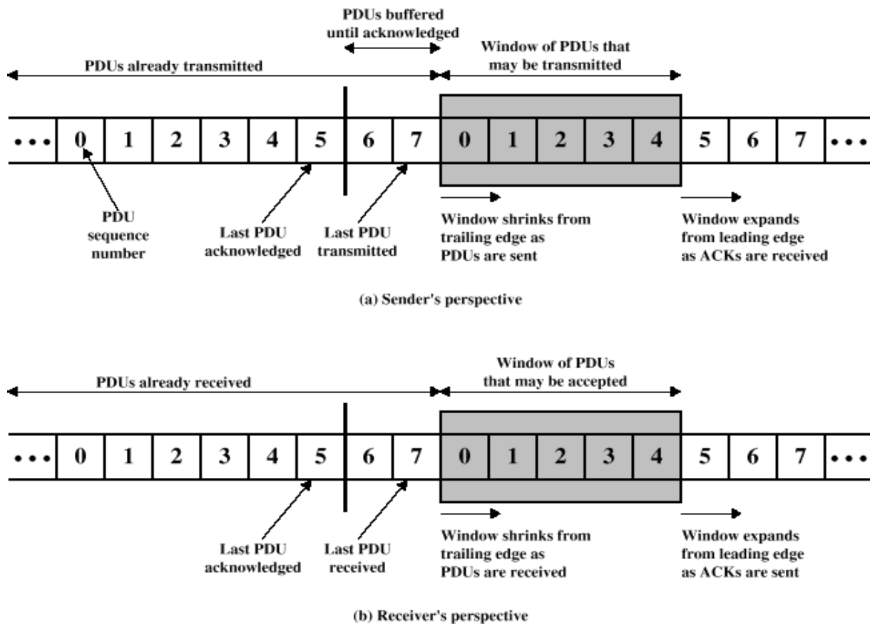
Figure 8.17 Sliding-Window Depiction
