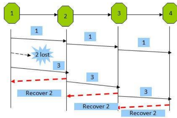
PSFQ Pump Operation. If not duplicate and in-order and TTL (T min < t < T max )
