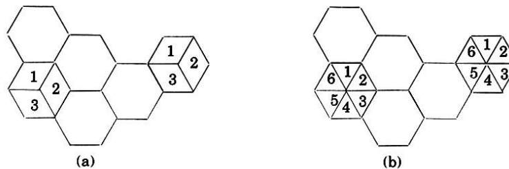
Figure 3.10 (a) 120° sectoring; (b) 60° sectoring.
