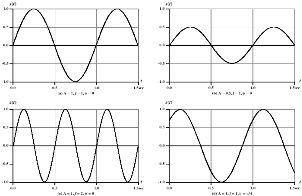
Figure 2.3 s(t) = A \sin(2\pi ft + \phi)
