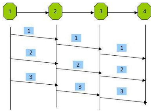
Error recovery – Store and Forward.
